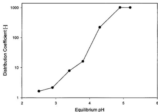
Fig. 3. The variation of distribution coefficients of \text{Sr}^{2+} ion with equilibrium pH of extracting solutions for the mixed extractant of \text{D}_2\text{EHPA} and \text{DCH18C6} in kerosene.
